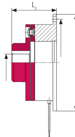
Hub on the outside (Variant 130)
