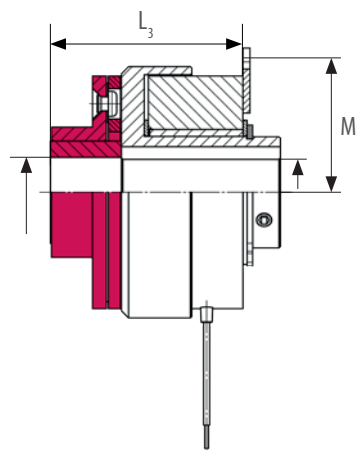
Hub with plain-bearing (Variant 640)
